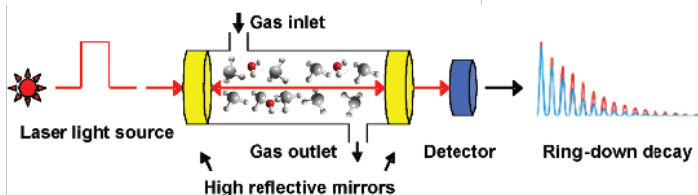
Advanced Cavity Ring-Down Spectroscopy to measure and control critical impurities.
