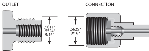
CONNECTION 170 LECTURE BOTTLE OUTLET – NON-CORROSIVE GASES .5625"-18 RH EXT. and .3125"-32 RH INT. using a Flat Seat with Washer
