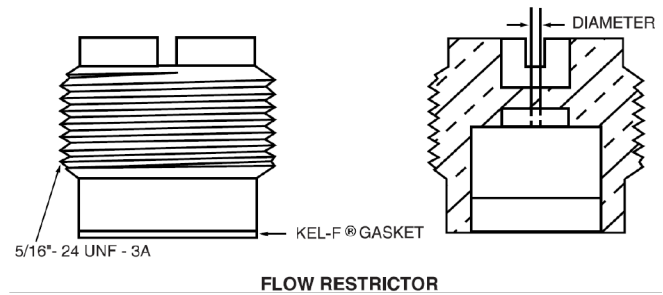
Figure 1: Restrictive Flow Orifice
